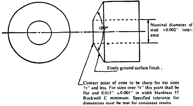
FIG. 2 Hardened Steel Cone
